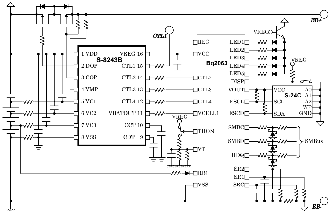
Figure 10 Application circuit 2
