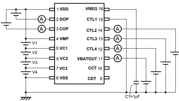
Test circuit 9
