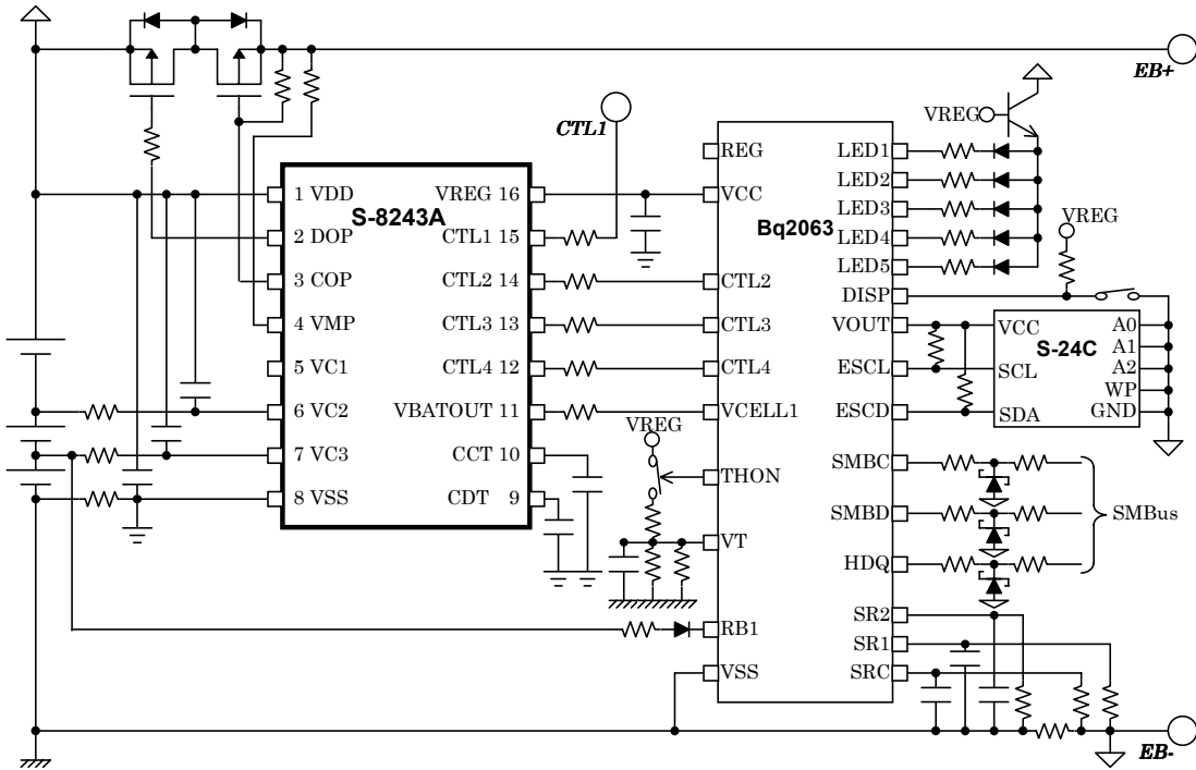
Figure 9 Application circuit 1
