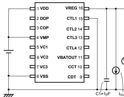
Test circuit 2
