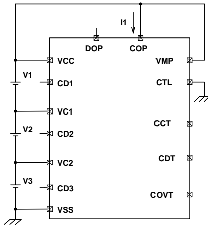
Masurement circuit 9
