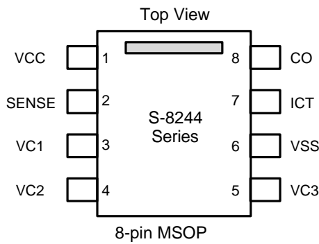
Figure 2 Pin Assignment
