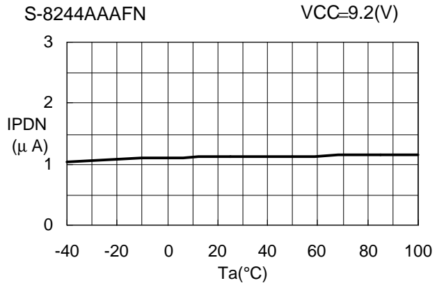
Current Consumption at Power Down vs Temperature
